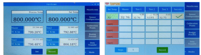
Main Screen
